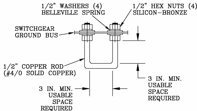
LINE & LOAD SIDE OF CURRENT TRANSFORMERS LINE SIDE POTENTIAL TRANSFORMERS
